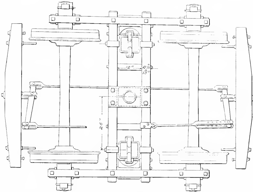
Fig. 4793. Plan of Truck.
